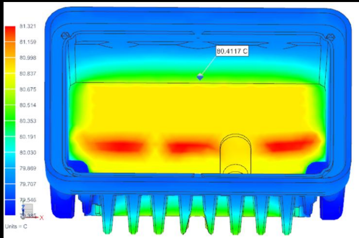
Heat Simulation Analysis
